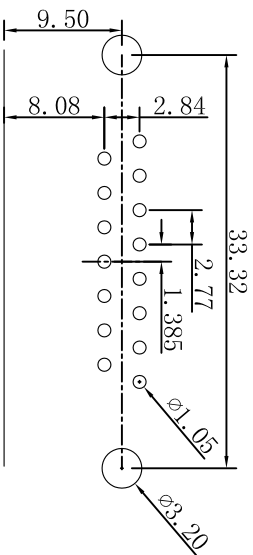
PCB Layout
